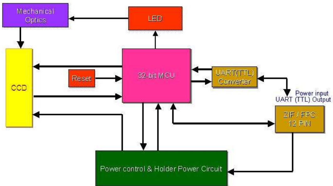
1-1. MT752 / MT752L Block Diagram
